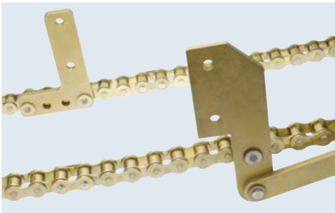
Roller chains with rocker arm and straight attachment Application: Instant coffee packaging equipment
