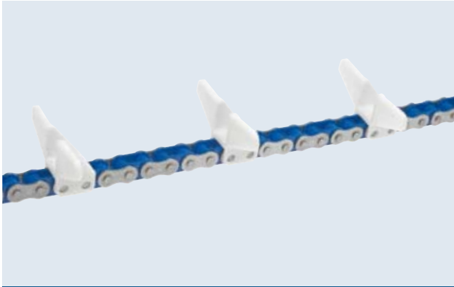
Roller chain with plastic inner links and special clips Application: Packaging industry
