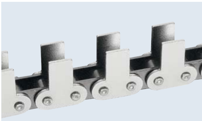
Special chain with plastic inner links and straight attachments on both sides Application: Laboratory techniques
