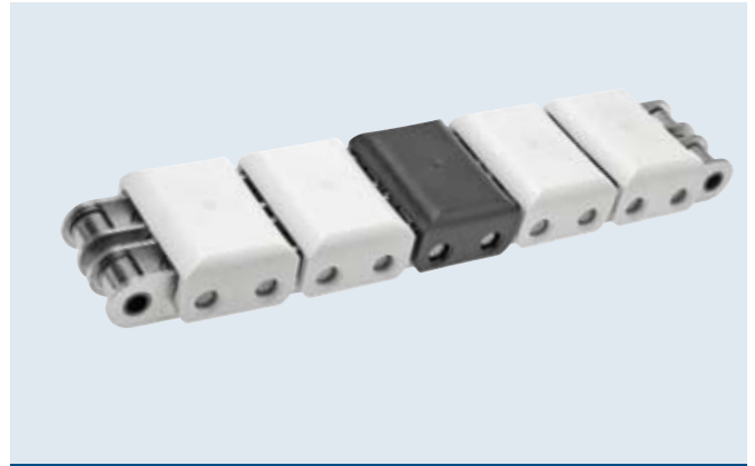
Duplex Marathon roller chain with straight plates and plastic clips Application: Careful conveying of sensitive goods
