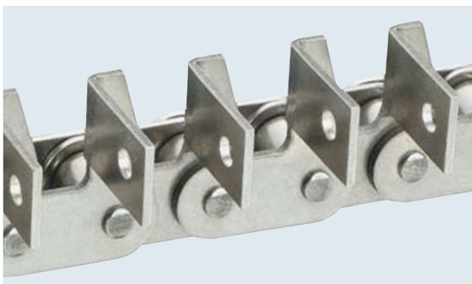
Roller chain stainless steel with straight and bent inner and outer attachments on one side Application: Materials handling
