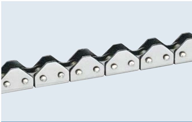
Roller chain with outer plates as U-clamp Application: Cosmetics industry
