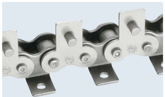
Roller chain stainless steel with bent or straight attachments on one side with pins Application: Materials handling
